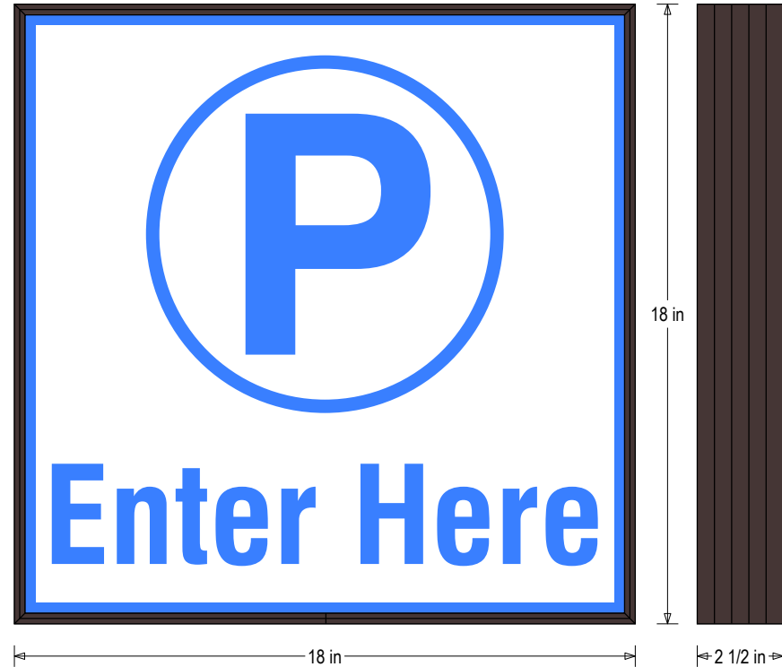
Frame Detail
