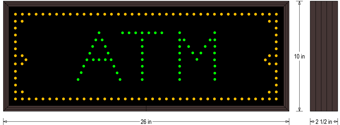
Frame Detail
